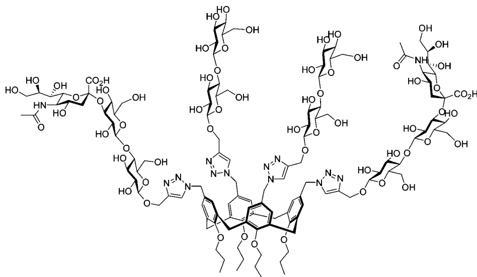
Figure 22. This impressive light harvesting antennae based on resonance energy transfer from the BODIPY branches to the core fluorophore was constructed in good yield using CuAAC.
