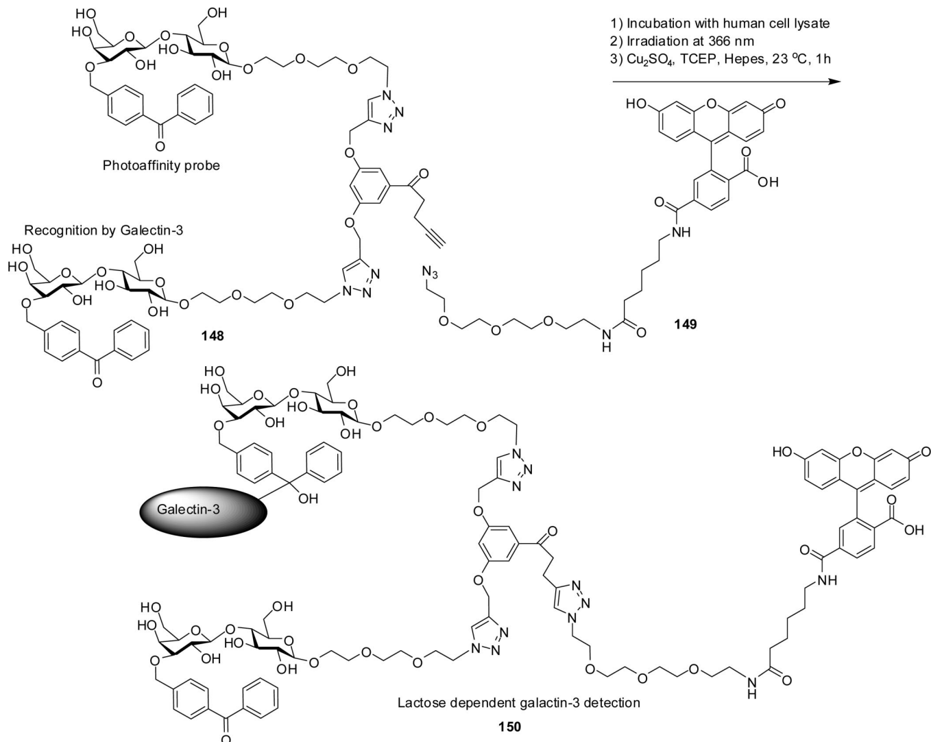
Figure 38. Selective labeling of galectin-3 in cell lysate. The photoaffinity probe reacts primarily with galectins, and separation by SDS-PAGE provides the bands for galectin-3 with selective suppression by increasing amounts of added lactose.
